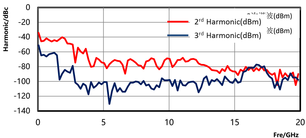
1466D-V Harmonic measured value
