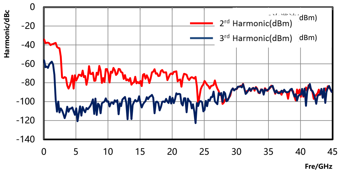
1466G-V Harmonic measured value
