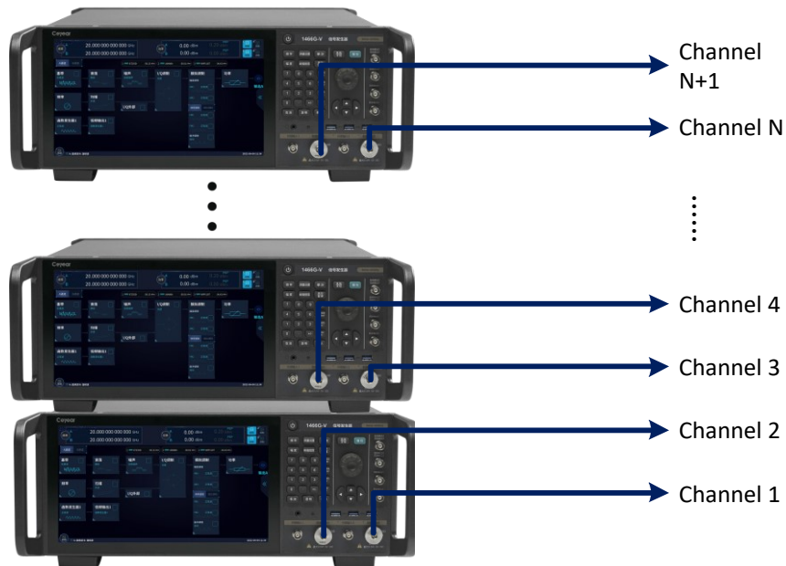
1466-V series signal generator multi-machine cascade
