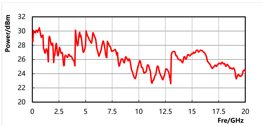
1466D-V Max.output power measured value (High power option H05-20)
