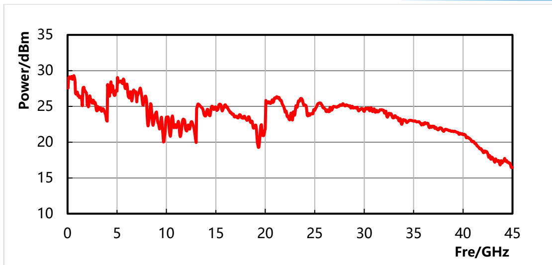
1466G-V Max.output power measured value (High power option H05-45)
