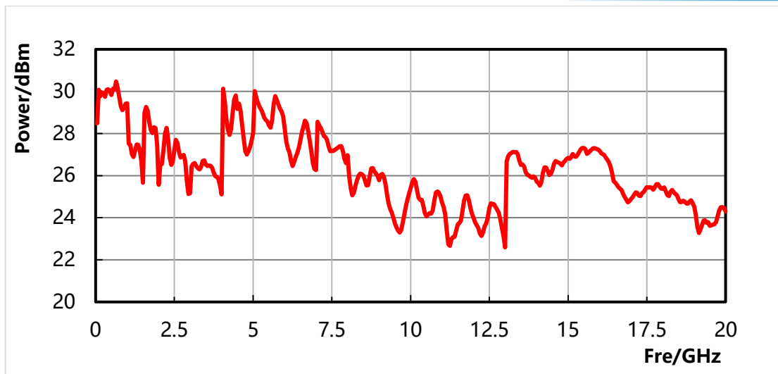
1466D max. output power measured value (large power option H05-20)
